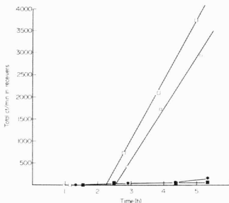
Fig. 1. Rates of auxin transport by internode segments (1 cm long; three segments per measurement) from 85-day-old cuttings of tomato plants. Circles, inverted; squares, control; open symbols, basipetal; filled symbols, acropetal.
